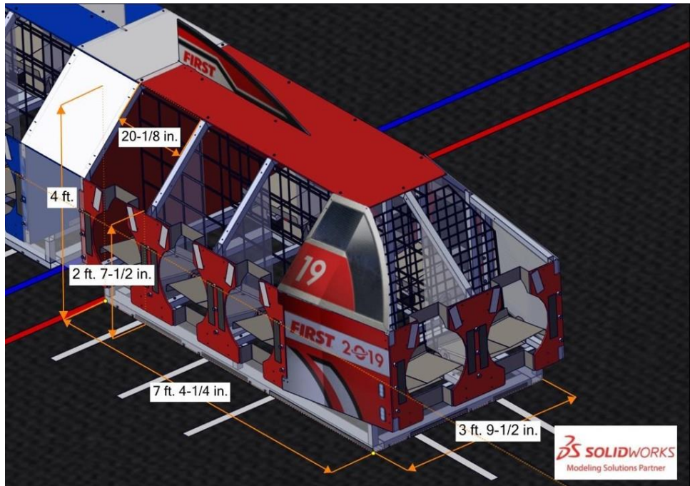
Figure 4-17 Major CARGO SHIP dimensions.
