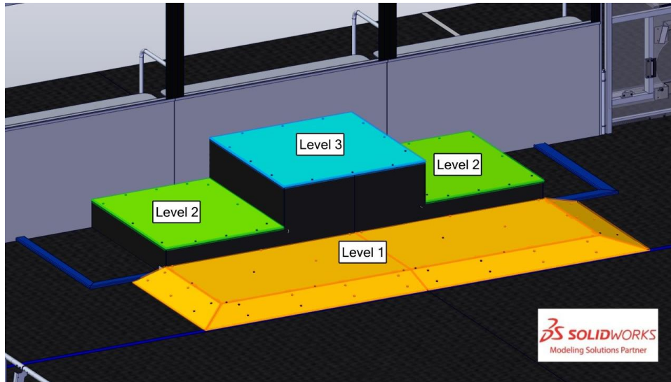
Figure 4-22 HAB PLATFORM Levels
