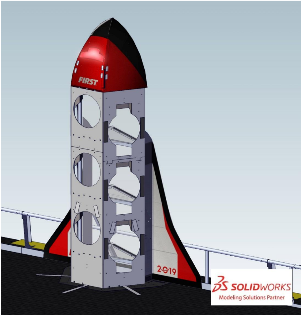
Figure 4-33 Complete Red ROCKET nosecone lit.
