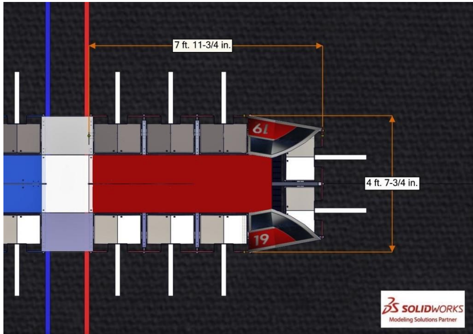
Figure 4-16 Overall CARGO SHIP length and width.
