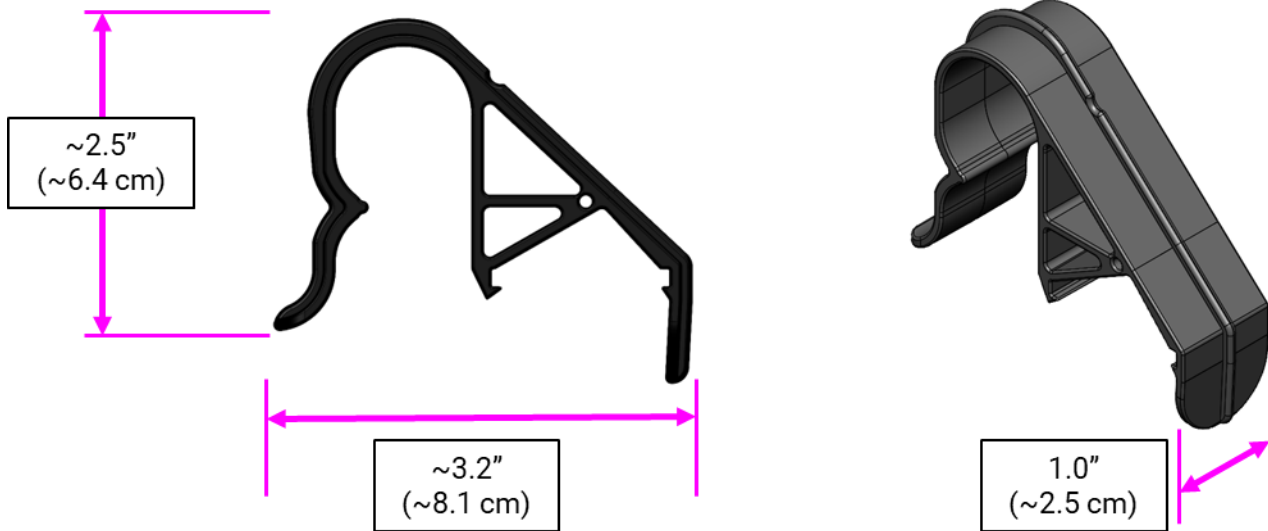
Figure 9-13: CLIP Dimensions
